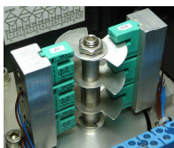
Ex i ... 8 V DC und 24 V DC induktive P+F-Sensoren, Ex eb mb ... / eb db ... 4 - 250 V AC/DC Soldo-Reed-Schalter, Ex 4 - 250 V AC/DC SPDT Bar-tec Schalter, 4 - 250 V AC/DC SPDT Crouzet-Schalter
