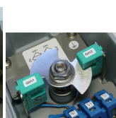
Ex i ... 8 V DC und 24 V DC induktive P+F-Sensoren, Ex eb mb ... / eb db ... 4 - 250 V AC/DC Soldo-Reed-Schalter, Ex 4 - 250 V AC/DC SPDT Bar-tec Schalter, 4 - 250 V AC/DC SPDT Crouzet-Schalter
